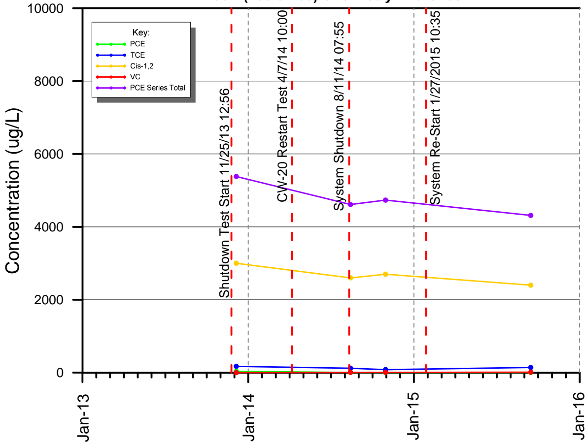
Figure 3.3-6 MW-136A (459.5-460) Chemistry - Ethenes
